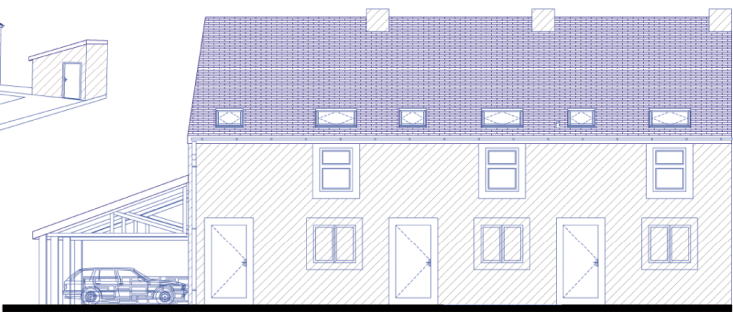
FACADE ENTREE
