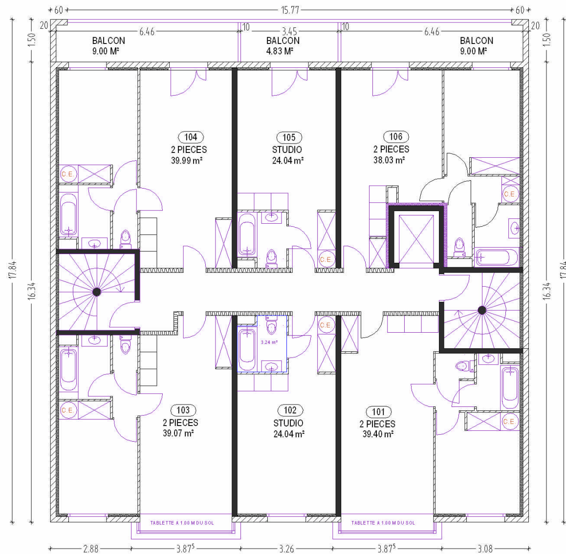
RESIDENCE ARGENTORA 3 BATIMENT A PLAN ETAGE 1
