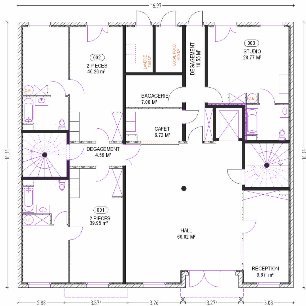
RESIDENCE ARGENTORA 3 BATIMENT A PLAN R.D.C.
