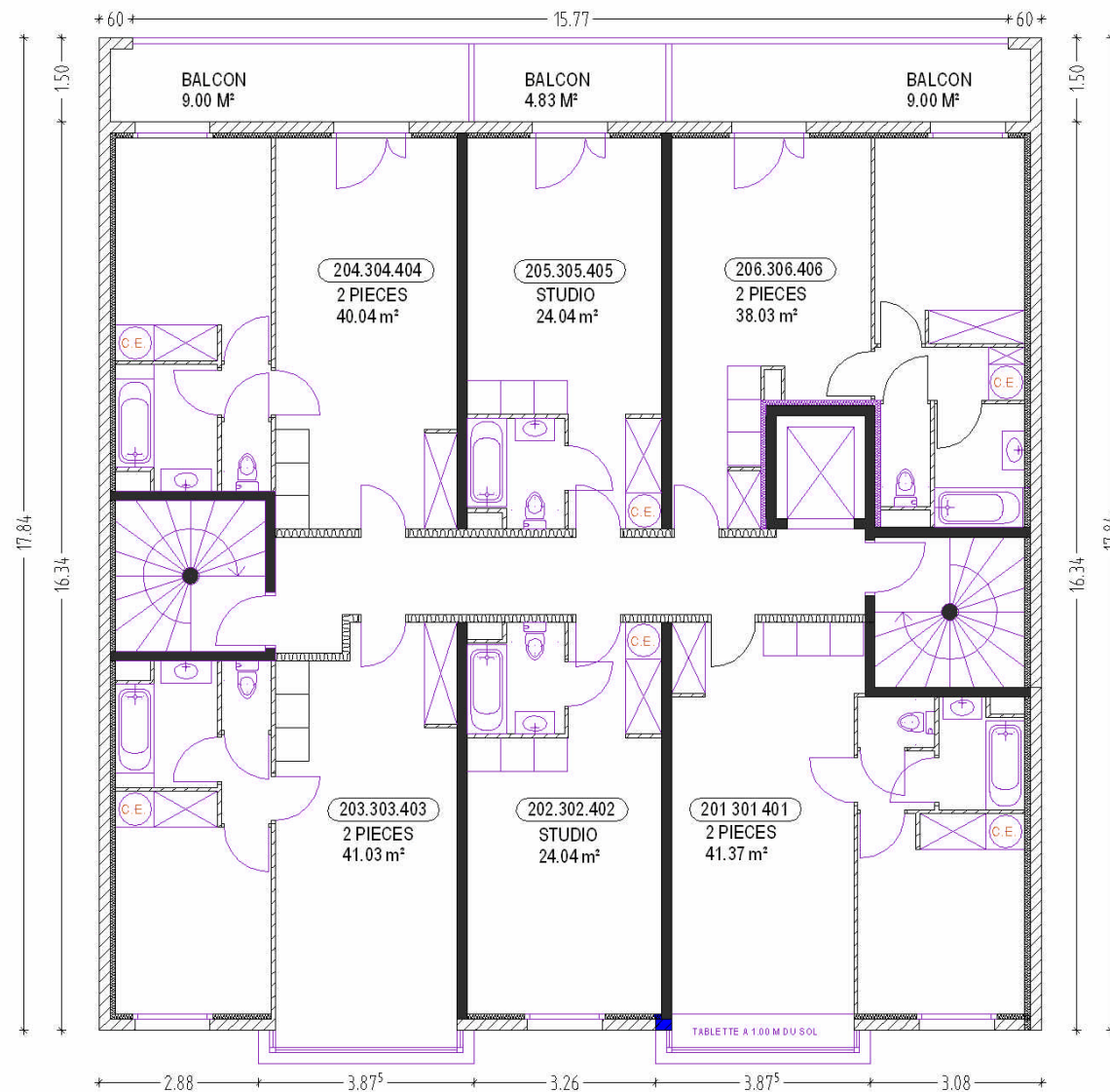
RESIDENCE ARGENTORA 3 BATIMENT A PLAN ETAGES 2,3,4
