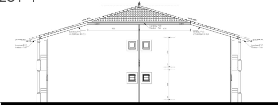
FACADE SUD
