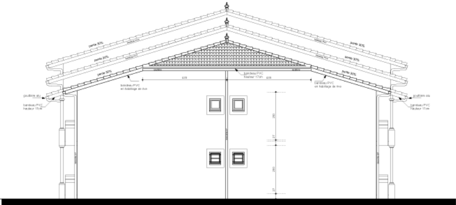
FACADE SUD
