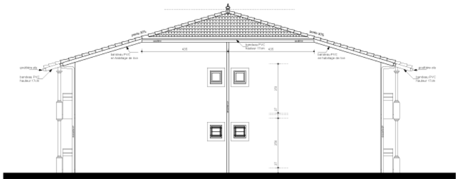
FACADE SUD
