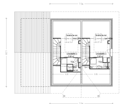
COMBLES
