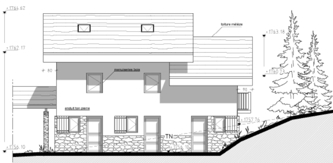
FACADE SUD
