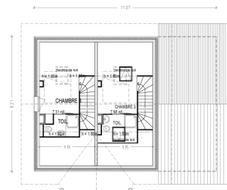
COMBLES
