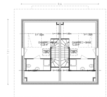
COMBLES
