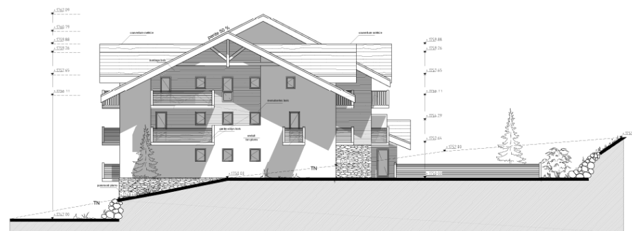
FACADE SUD
