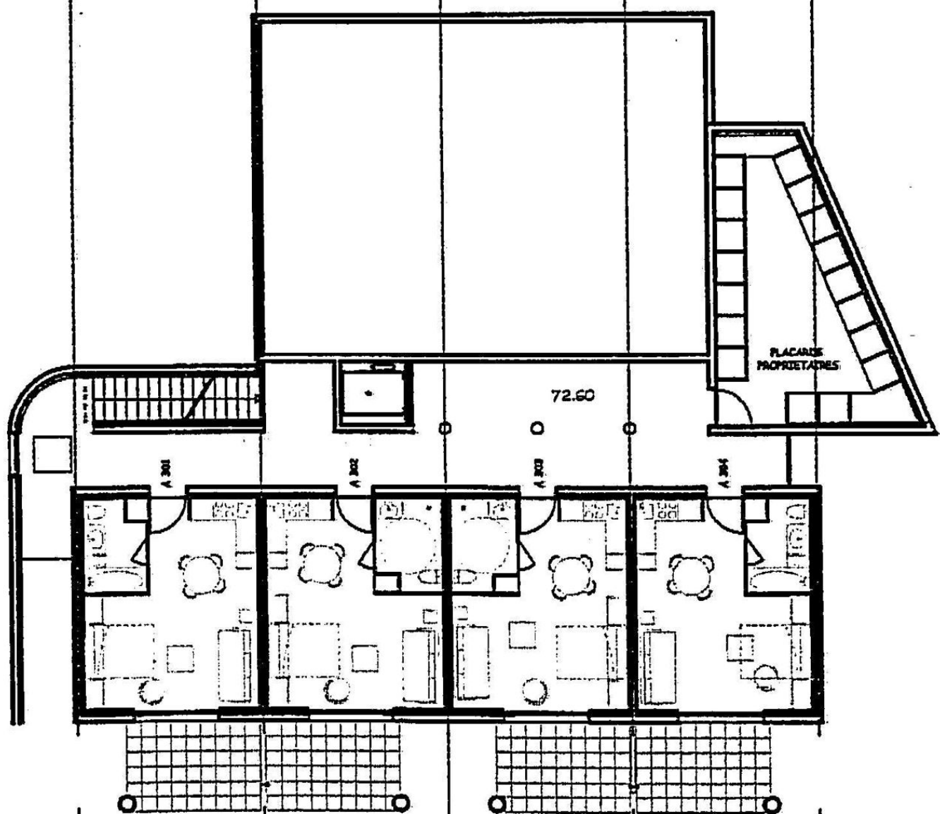
BATIMENT A NIV. 72.70
